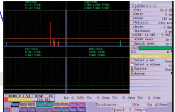
Display mode: Multi A-Scan
